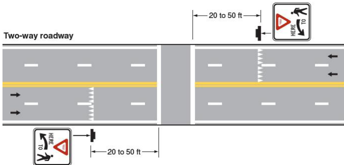
Mid-block crosswalk
